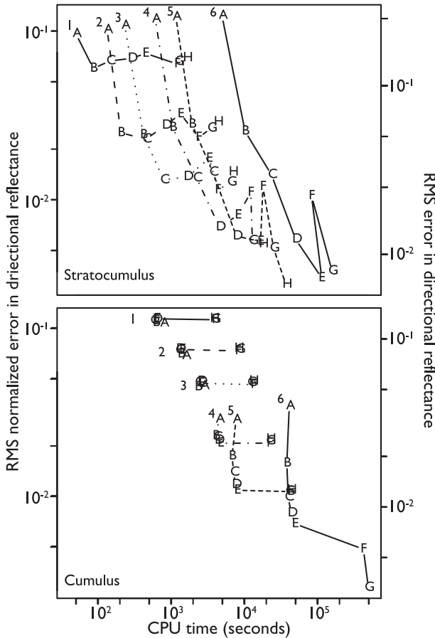
FIG. 7. Error in directional reflectance (intensity) computed using SHDOM as a function of total computation time for the stratocumulus and cumulus scenes. Both axes are logarithmic. Letters refer to spatial resolution and numbers (and line types) to angular resolution detailed in Table 2. Error is computed as the RMS difference over all directions and all pixels from the benchmark (6H) calculation. Values on the left axis are computed by normalizing the error by the domain mean in each direction before computing the RMS over directions; the right axis shows the RMS over direction of the raw error. When calculations in the cumulus scene use low angular resolution (cases 1–4), increased spatial resolution increases computation time without increasing accuracy, so points A–E are clustered to the left and F–H are on the right.
