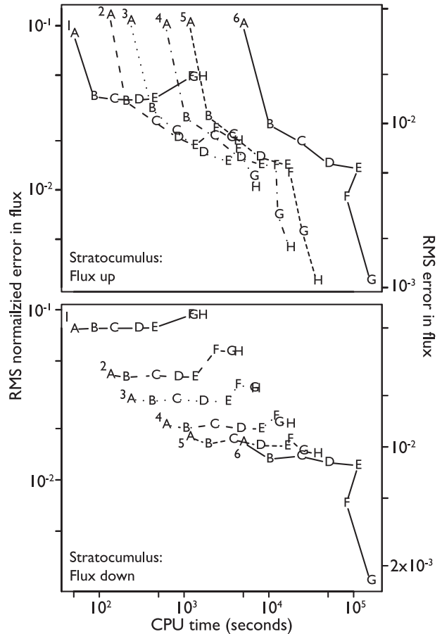
FIG. 8. Error in flux calculations, measured as the RMS difference from the benchmark (resolution 6H) over all pixels, as a function of total CPU time in the stratocumulus scene for upwelling flux at the domain top and downwelling flux at the surface. The RMS flux difference normalized by the domain mean flux is shown on the left axis; absolute values are on the right. Accuracy in downwelling flux depends mostly on angular resolution; accuracy in upwelling flux depends on spatial resolution as well.
